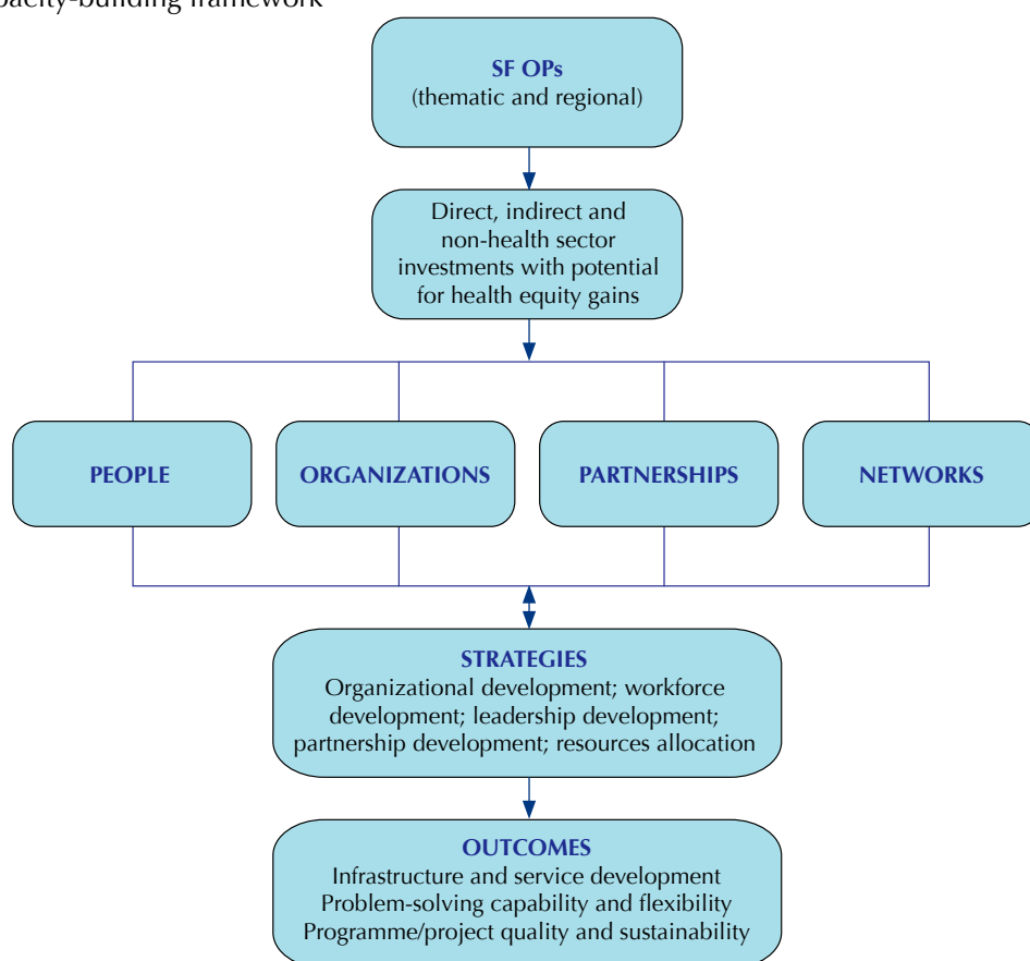
Fig. 3. Capacity-building framework
